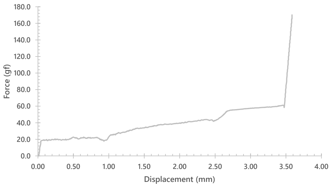
Logitech Long Hua Purple (Condenser) (Upstroke)
